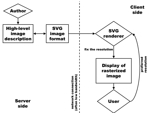
Figure 5: The process of delivering a resolution-independent SVG image across the network.
