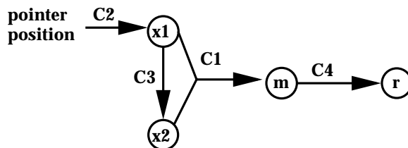
Figure 3: One-way (directed) constraint graph for Figure 2.
